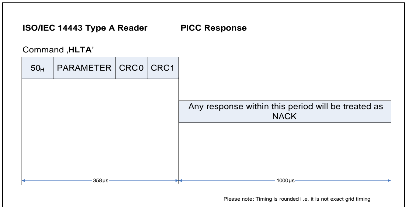
Figure 29 HLTA Command
